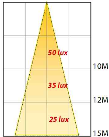
Neutral White @ 200W
