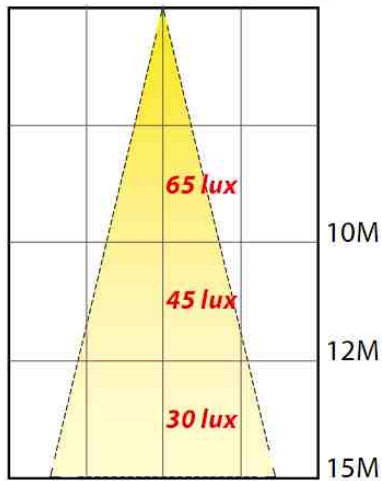
Cool White @ 200W
